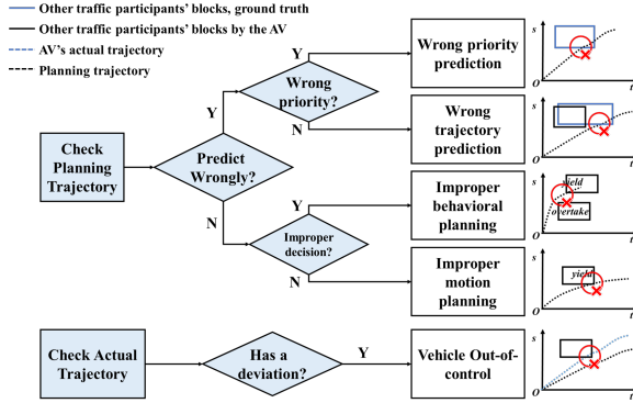
Figure 5: CAT for causality analysis
