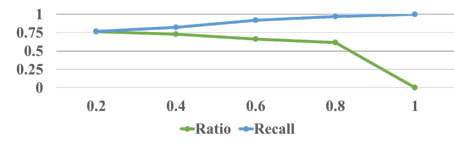
Figure 6: Ratio (higher is better) and recall (higher is better) of the pruning method under different thresholds
