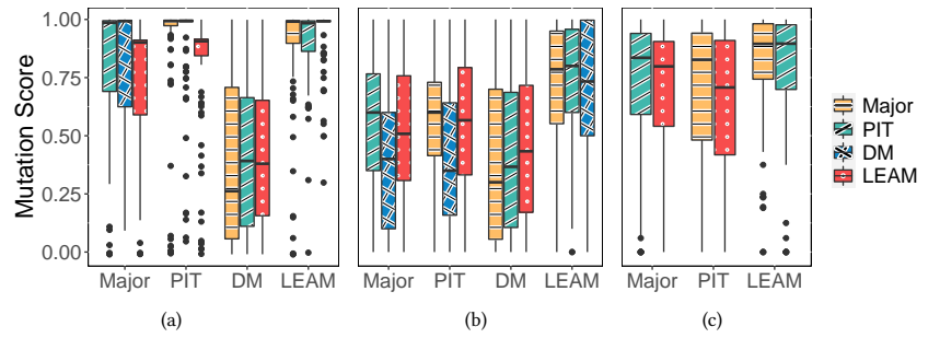
Figure 3: Ability of representing mutation faults constructed by other mutation techniques. (a) shows the result when using all the constructed mutation faults; (b)/(c) shows the result under controlling for the number of mutation faults when considering/ignoring DeepMutation (DM).
